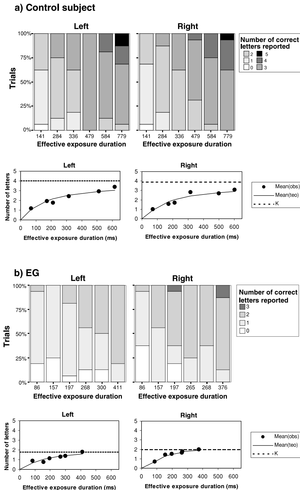
Fig. 6. Whole report performance in the left and the right hemi-field (a) for a typical control subject (aged 40 years), representing the performance of the control group ( K_{left} = 4.0 , K_{right} = 3.9 ; C_{left} = 29 , C_{right} = 24 ) and (b) for patient EG. The upper half of each panel shows, separately for each visual hemi-field and effective exposure duration, the proportion of trials on which 0, 1, 2, 3, 4, or 5 letters were correctly reported. The lower half of each panel presents the mean number of correctly reported letters as a function of effective exposure duration, separately for each visual field. Filled circles indicate observed values, solid lines represent the best fits of the observed scores by the TVA model. The origin of each curve was normalized to the perceptual threshold t_0 . The estimate of the visual working memory capacity K is marked by a dashed horizontal line. (teo: theoretical; obs: observed).
